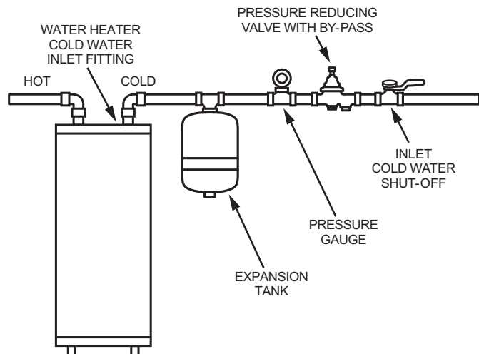
RECOMMENDED INSTALLATION - VERTICAL MOUNTING
